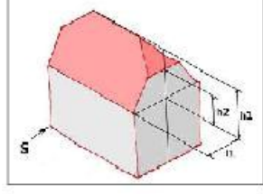
2.3 = half-hipped
